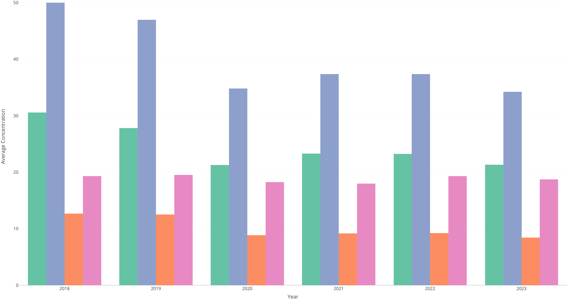
Yearly Average of Air Pollutants
